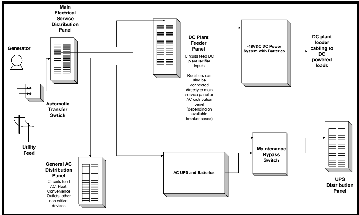
Figure #4: Typical Headend General One-Line Diagram
