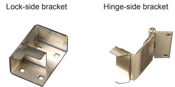
Fig. 4, Bracket detail
