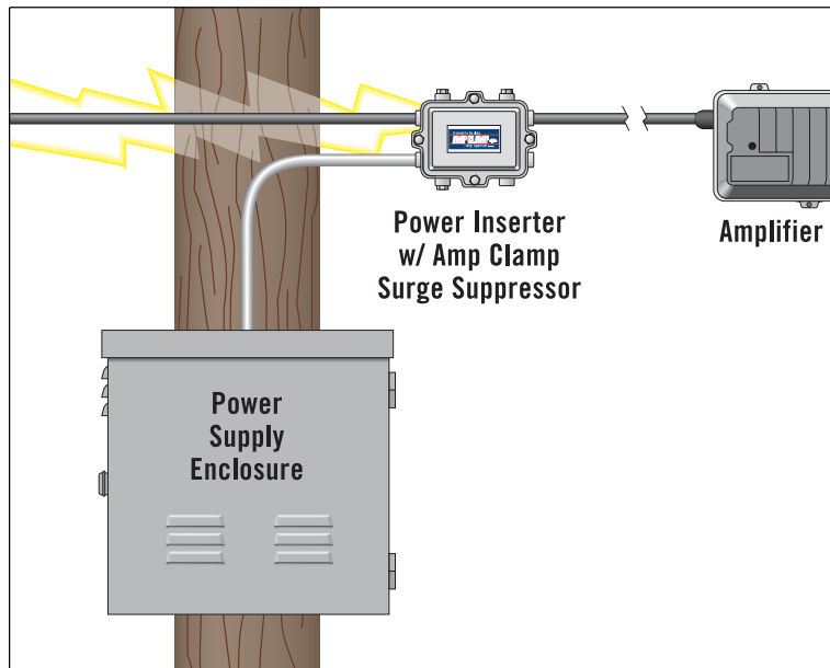
FIGURE 1: Broadband Power System With Surge Protection
