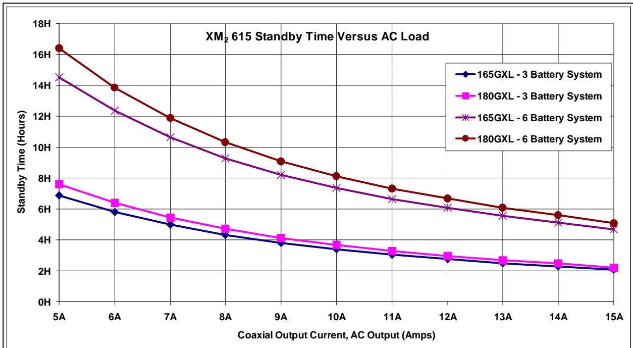
Figure 5. AlphaCell 180GXL and 165GXL battery run times for different XM 2 output currents loads into the CATV plant.
