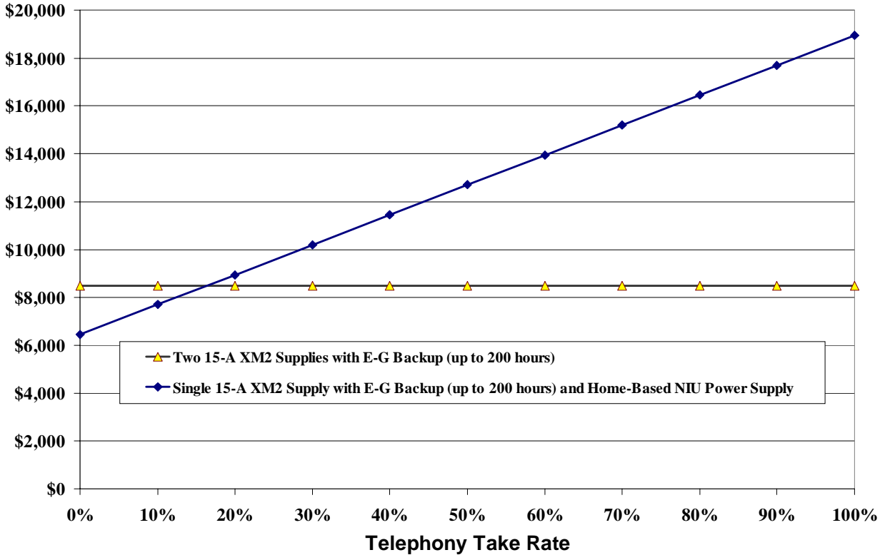
Figure 2. NIU powering alternatives: network powering or home-based powering, with backup provided by an E-G.
