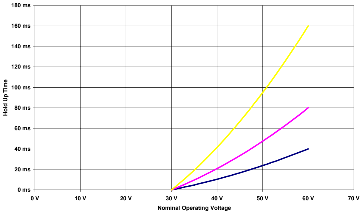
Figure 4. Three examples of holdup times as a function of network operating voltages. At a 60-V operating voltage, three different holdup times are shown: 40ms, 80ms, and 160ms. Note that all three decrease dramatically at lower operating voltages.
