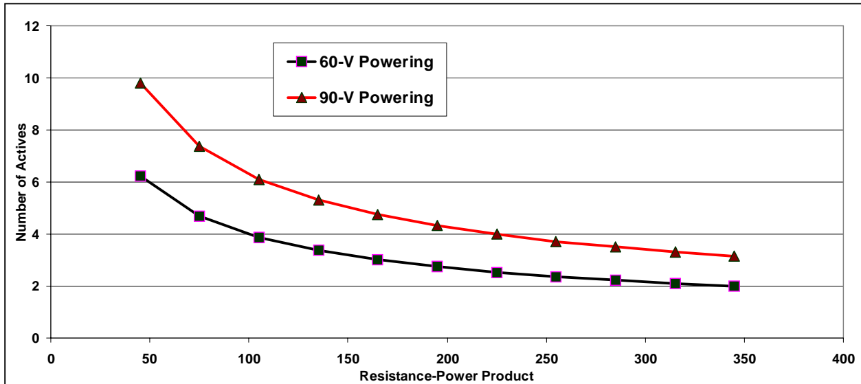
Figure 6. Increase in the number of actives in a string produced by changing from 60-V powering to 90-V powering. The resistance-power product refers to the coaxial resistance between actives and power is the constant-power load of the active.
