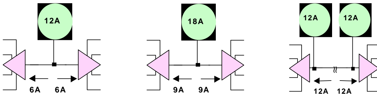
Figure 3. Increasing power into network for powering telephony NIUs. From a single 15-A supply providing 12-A to the network, to a 22-A supply providing 18-A of network power, to two 15-A supplies with a total of 24-A of network current.
