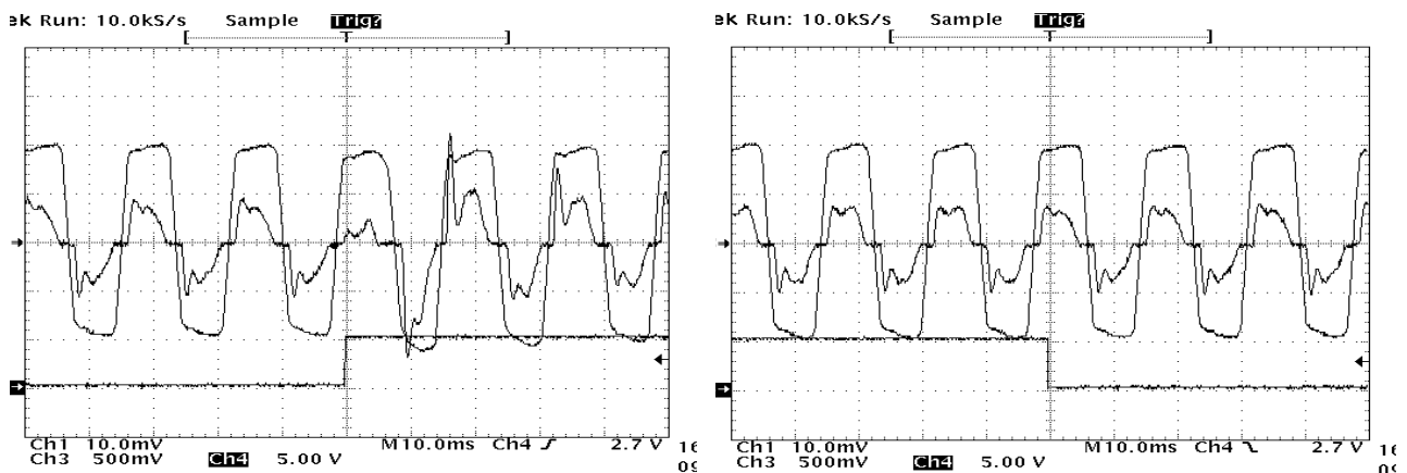
Figure 1. Examples of XM_2 transitions between utility powering and standby powering using CATV load.
