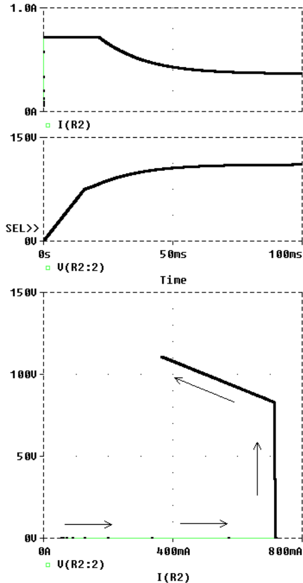
Figure 7. Startup simulation with a 40-W ONU load, R_W = 80\Omega , L_W = 2.4\text{mH} , and C_{ONU} = 150\mu\text{F} . Lower figure is the state-space trajectory with inductor current on the horizontal axis, and capacitor voltage on the vertical axis.
