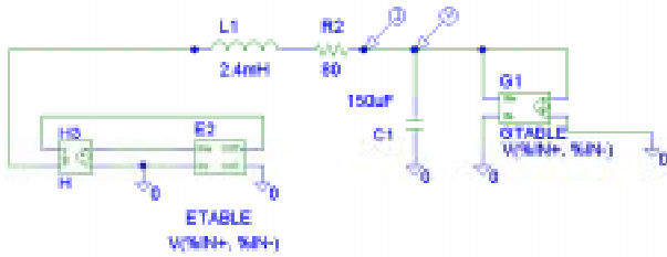
Figure 6. Pspice circuit for state plane simulations.
