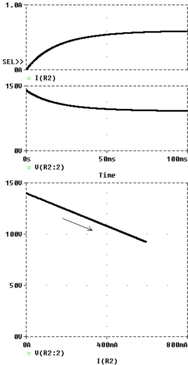
Figure 10. Delayed ONU startup with initial conditions of 140V and 0A, for a 55-W ONU load.
