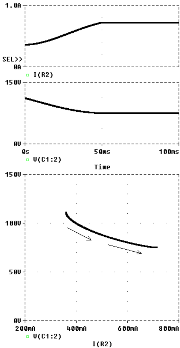
Figure 12. Transient response to step change in ONU load from 40W to 55W with a larger twisted-pair inductance L_W = 1.3H .
