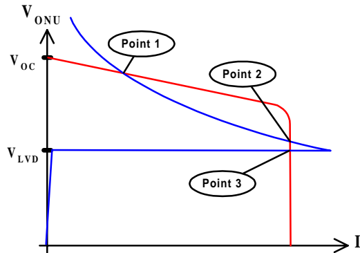
Figure 4. Combined RPS and winding resistance plotted with ONU load characteristics.
