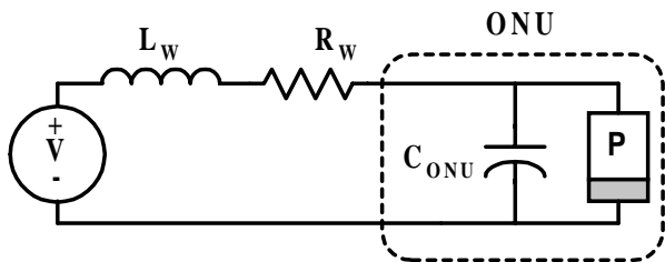
Figure 1. Equivalent circuit of RPS-ONU system. The rectangle enclosing the letter “P” represents the constant-power load of the ONU. Inductance L_W and resistance R_W represent the characteristics of the copper twisted pairs which interconnect the RPS and ONU.
