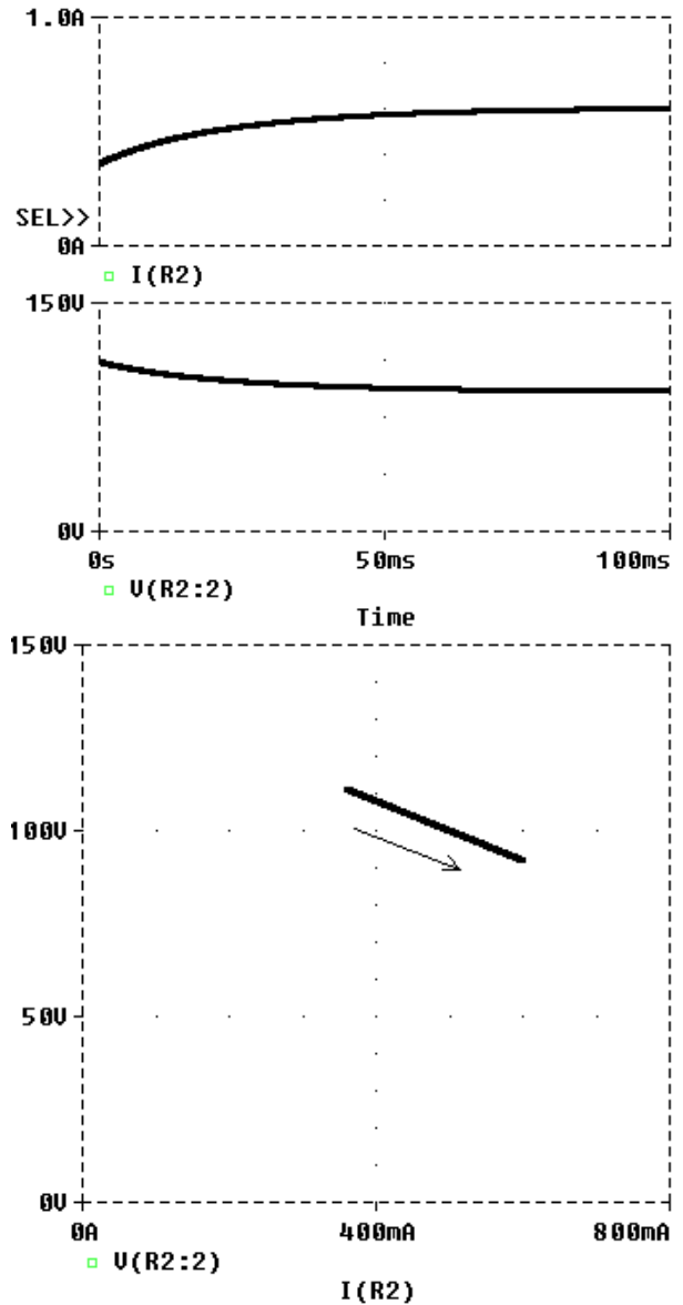
Figure 11. Step change response for an ONU power change from 40W to 55W.
