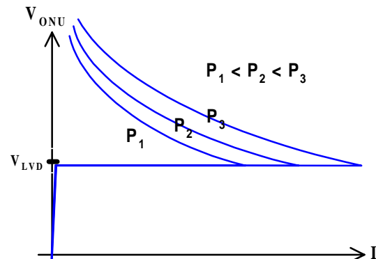
Figure 2. Graph of ONU V-I characteristics for three different ONU power loads. Higher ONU powers are characterized by a larger V-I product and are located higher and to the right on V_{ONU} -versus- I plane.
