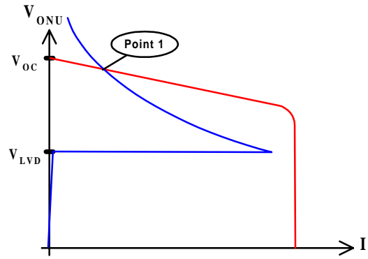
Figure 5. Same data as Fig. 4 with lowered ONU power load. Note absence of equilibria at points 2 and 3.
