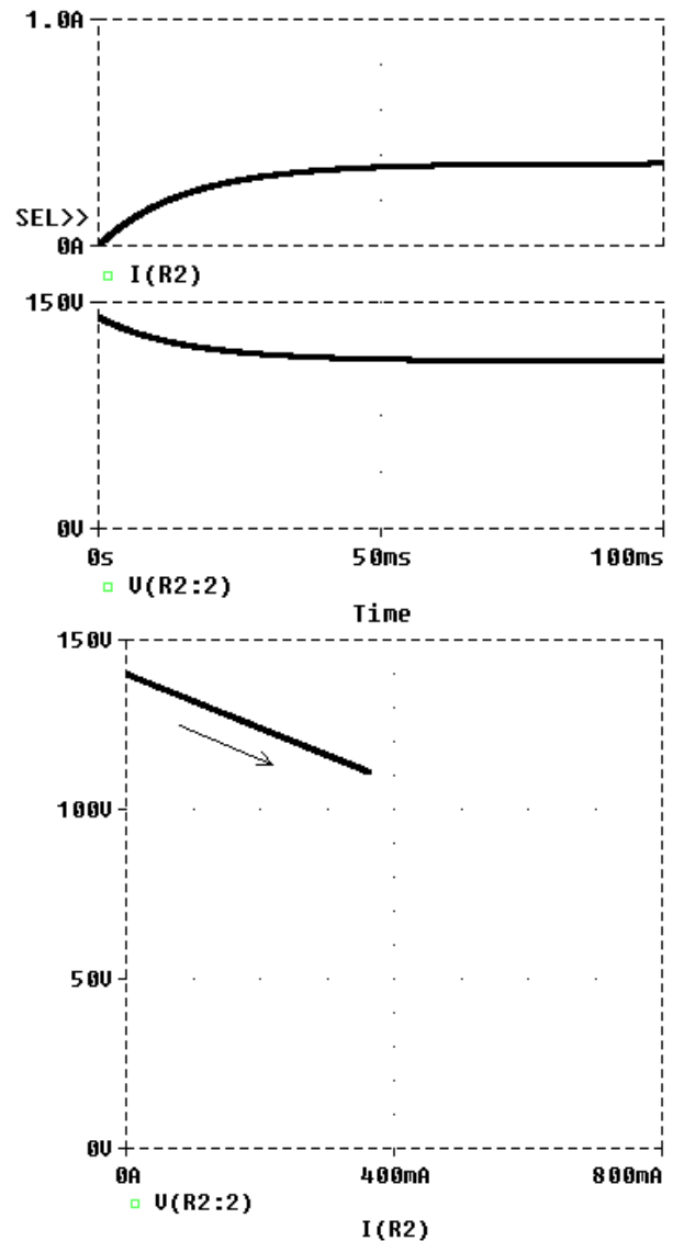
Figure 9. Delayed ONU startup with initial conditions of 140V and 0A, for a 40-W ONU load. Lower figure is the state-space trajectory with inductor current on the horizontal axis, and capacitor voltage on the vertical axis.
