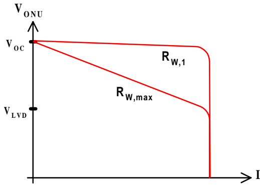
Figure 3. Combined characteristics of current-limited RPS source and copper-pair winding resistance R_W . Longest possible RPS-ONU line shown as R_{W,max} while characteristics from a short RPS-ONU distance is seen with R_{W,1} .
