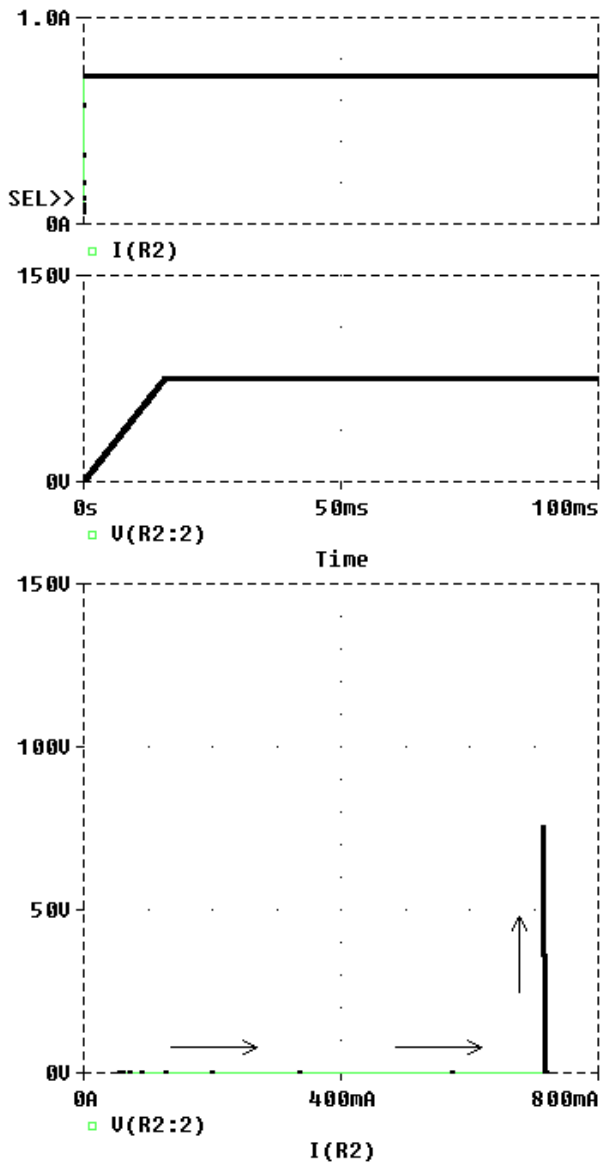
Figure 8. Startup simulation with a 55-W ONU load. Lower figure is the state-space trajectory with inductor current on the horizontal axis, and capacitor voltage on the vertical axis.
