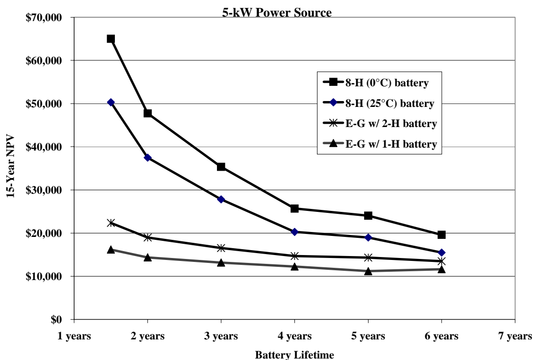
Figure 5. Fifteen-year net present value analysis which compares eight-hour battery plants, sized for eight-hour backup at both 25°C and 0°C. Telecom genset examples assume a one-hour and two-hour battery plant together with the genset.
