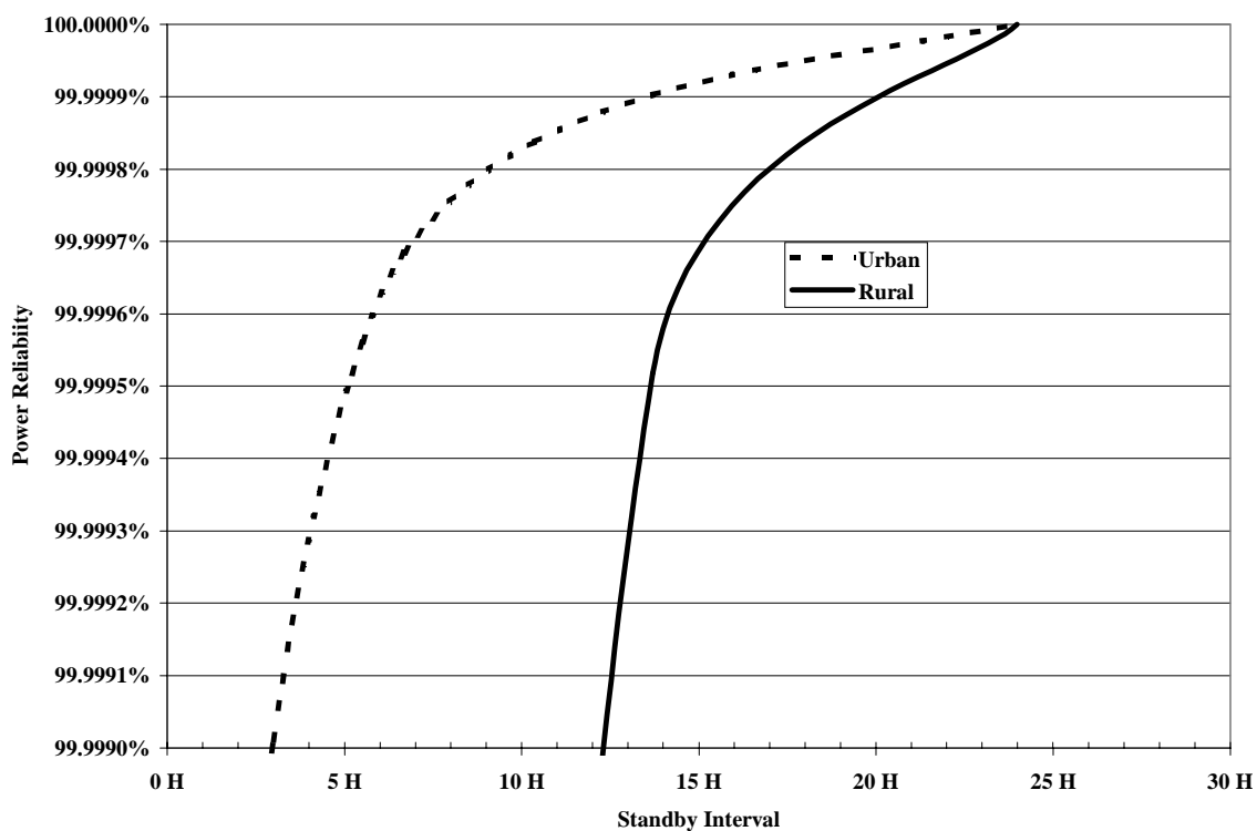
Figure 3. Same data as Fig. 2, with a change in scale for the power reliability to illustrate power reliability between five and six nines.
