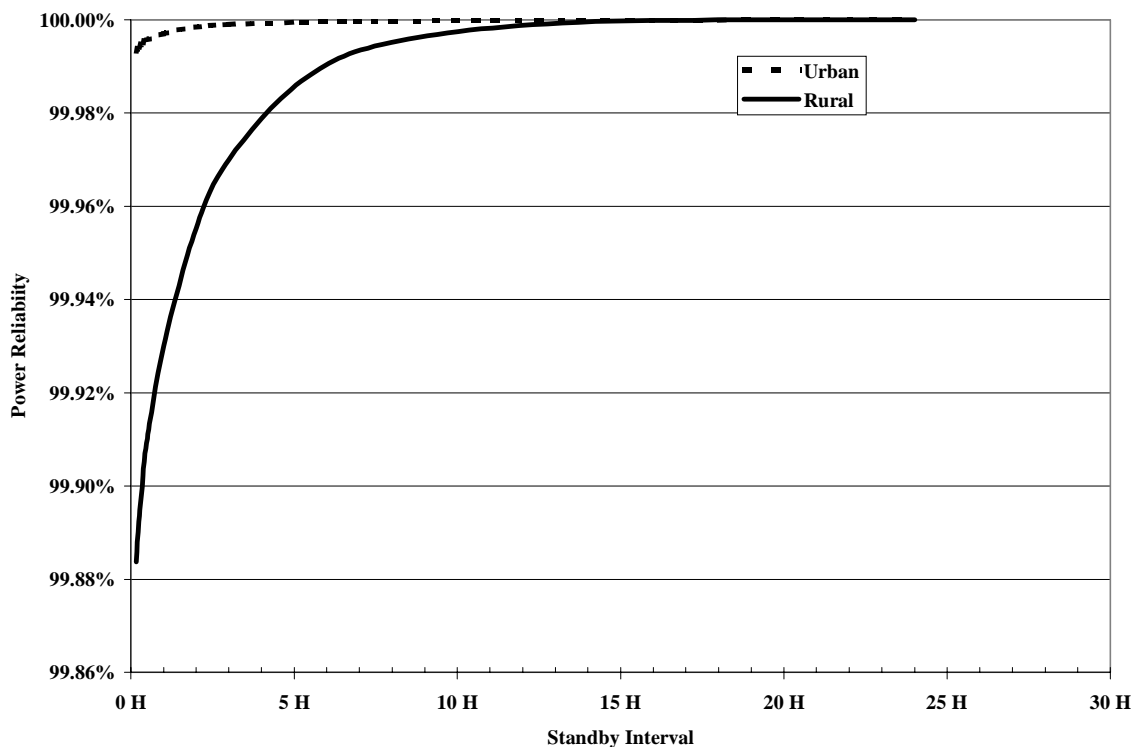
Figure 2. Powering reliability as a function of the powering standby interval. Statistical data does not include data for outages in excess of 24 hours, so reliability with a 24-hour genset is 100 percent.
