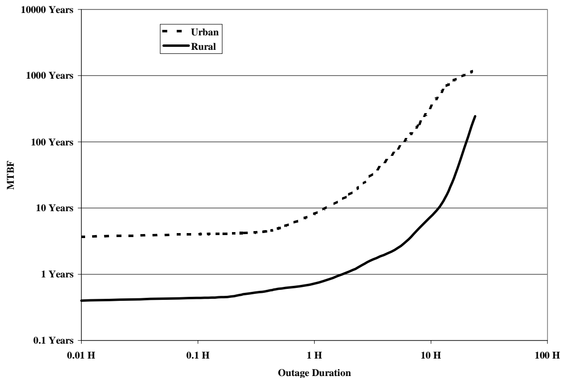
Figure 1. From [5], reliability of 240-Vac mains in urban and rural areas of the UK.
