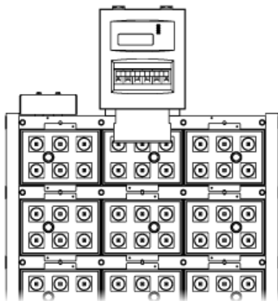
Illustration of DCX Series Mounting Kit (Shown installed on EnerSys DDmP 125-33)
